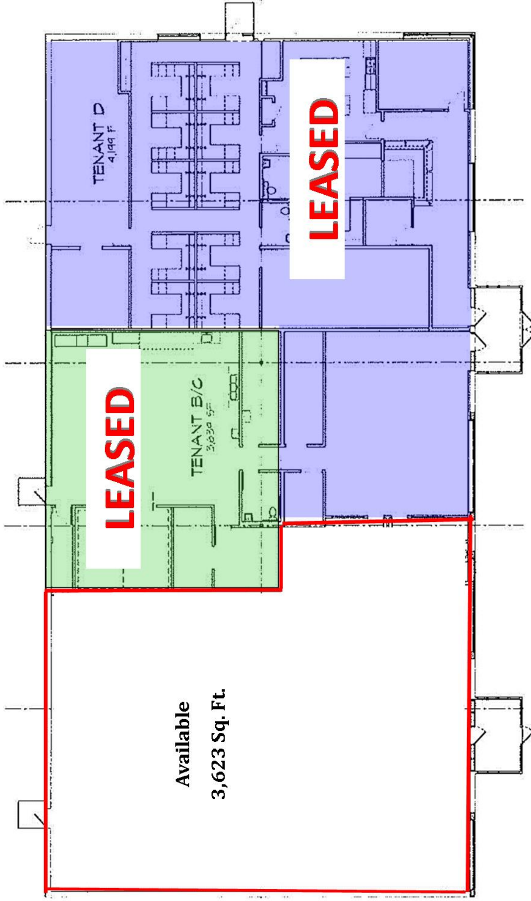
2 FLOOR PLAN 1/8" = 1'-0" 12,244 GROSS S.F.
